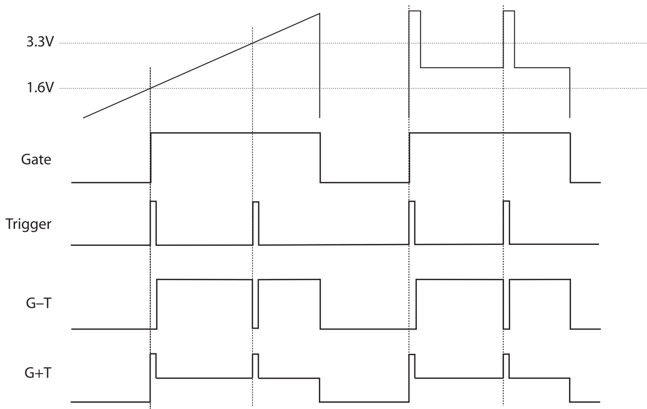
Analogue Waveform
